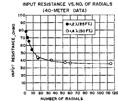
Fig. 2 -- Input resistance of a quarter-wave ground-mounted resonant vertical as a function of the number of radials.
