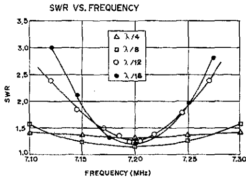
Fig. 4 — Standing wave ratio of various short verticals compared to a resonant quarter-wave antenna. The sixteenth wavelength antenna is the 8-1/2-foot helical design, the twelfth wavelength is the 10-foot antenna, and the eight wavelength is the 15-foot, 10-inch antenna. (All three are described in the text.)
